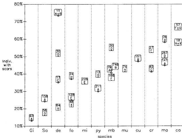
Fig. 1: Proportion of scarred individuals in 10 Lithobius -species and 2 species of Geophilomorpha from various locations in West-Germany. Letters in the boxes refer to the collections listed in Table 1. Numbers indicate the sample sizes. Calculations for hand-collected samples (rounded boxes and open-circle marks) are based on adults ( \geq PL 5) only. The sample of Lithobius dentatus for (A + B) contains stage PL 4. Species codes: ca Lithobius calcaratus C.L. KOCH, cr L. crassipes L. KOCH, cu L. curtipes C.L. KOCH, de L. dentatus C.L. KOCH, fo L. forficatus (L.), ma L. macilentus L. KOCH, mb L. mutabilis L. KOCH, mi L. microps MEINERT, mu L. muticus C.L. KOCH, py L. pygmaeus LATZEL, Gi Geophilus insculptus ATTEMS, Sa Strigamia acuminata LEACH.
